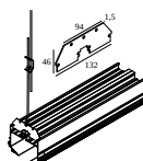
420 52 98 01 SPM52 - SUSPENSION BRACKET
