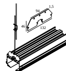
420 52 98 01 SPM52 - SUSPENSION BRACKET
