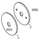
204 00 90 COVERSET R 90
