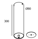
418 48 100 SUPERLOOP POWERBOX H - 48V-DC / 100W
