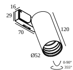
20583 9040 SUPERLOOP-SPY 52 SOFT 93030 MDL
