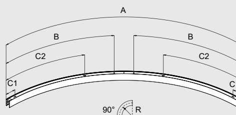
CURVE R1675/90°
