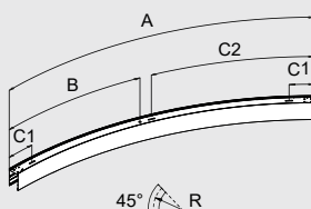
CURVE R1675/45°
