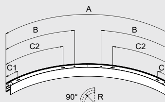
CURVE R840/90°
