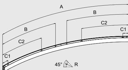
CURVE R2925/45°
