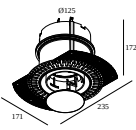
29810 0200 MOUNTING KIT TOP AIR ONLY 1
