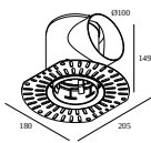
29810 0010 MOUNTING KIT SIDE AIR 101
