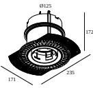
29810 0210 MOUNTING KIT TOP AIR 101
