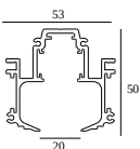
420 20 10 00 SPM20 - PROFILE 1m
