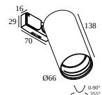
20569 9210 SUPERLOOP-SPY 66 92718 MDL
