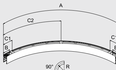
CURVE R840/90°
