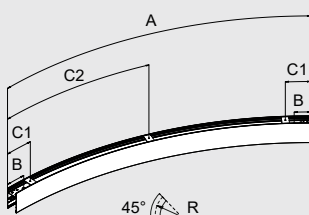
CURVE R1675/45°
