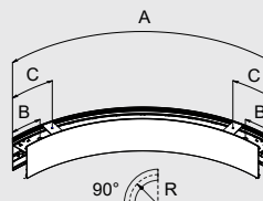
CURVE R420/90°
