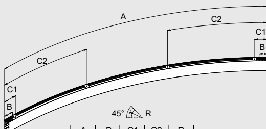
CURVE R2925/45°
