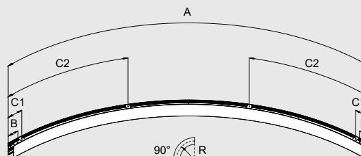
CURVE R1675/90°
