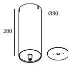
418 48 050 SUPERLOOP POWERBOX L - 48V-DC / 50W
