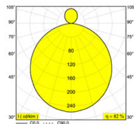
MULTINOVA R05 DOWN-UP
