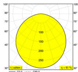
MULTINOVA R05 DOWN
