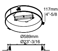
MULTINOVA 55 RECESSED KIT
