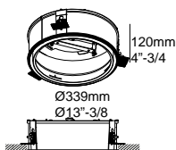
MULTINOVA 30 RECESSED KIT
