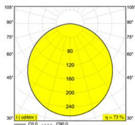
MULTINOVA R03 DOWN
