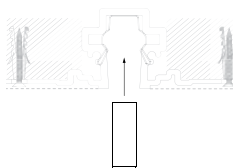
TGL-TR - PROFILE + TGL-LEDLINE - PROFILE
