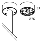
422 99 01 B XY180 CONNECTION BOX B
