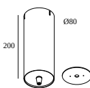
418 48 050 SUPERLOOP POWERBOX L - 48V-DC / 50W
