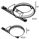
21032 0220 SOLI - VOICE COMMAND GOOGLE HOLDER
