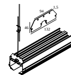
420 52 98 01 SPM52 - SUSPENSION BRACKET
