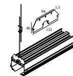
420 52 98 01 SPM52 - SUSPENSION BRACKET
