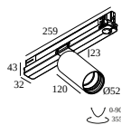
19881 9025 SPY 52 TW 96520 ADM DIM5
