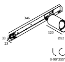
19886 9205 SPY 52 WALLWASH 927 ADM SLIM DIM5
