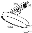
27937 9305 MULTINOVA 30 PIVOT SMOKE 930 ADM DIM5
