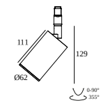
421 152 811 92 MDL M20/M26 - SPY FOCUS 927 MDL
